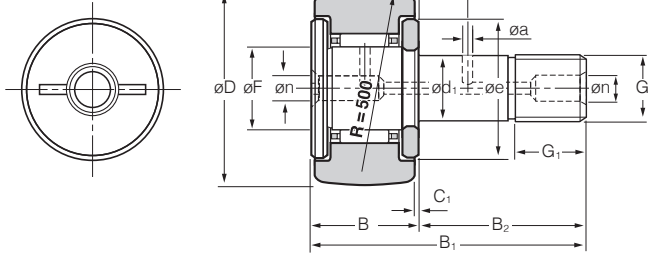
KR (with cage)
