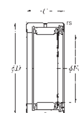
RNA49 -- L (with single seal)
