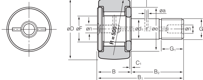
KRV (full-complement roller type)
