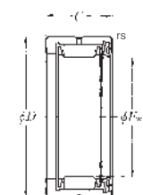
RNA49 -- L (with single seal)
