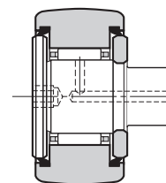
KR -- LLH (with cage, sealed)
