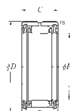
RNA49 -- LL (with double seal)
