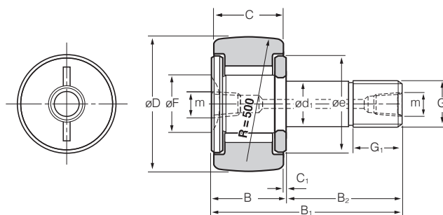
KRVT (full complement)
