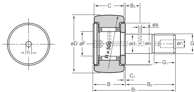
KR -- H (with cage)
