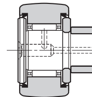
KR -- LL (with cage, sealed)
