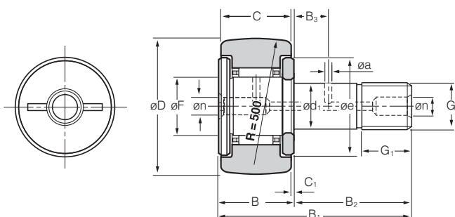
KR (with cage)
