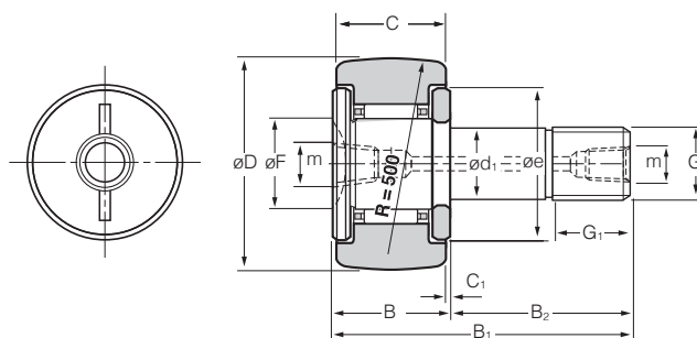
KRT (with cage)
